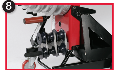
Central Pivot Point Balanced pivoting for easy switching between horizontal and vertical position.
